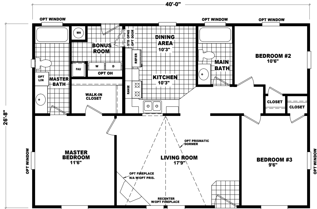
MODEL: CS4028A APPROXIMATELY 1066 SQ. FT. 3 BEDROOM, 2 BATH
