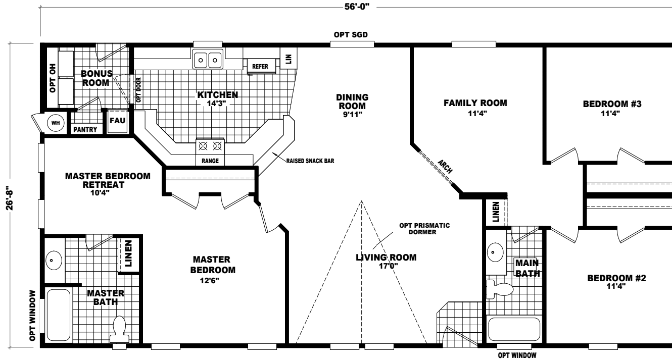
MODEL: GS-2568K APPROXIMATELY 1493 SQ. FT. 3 BEDROOM, 2 BATH
