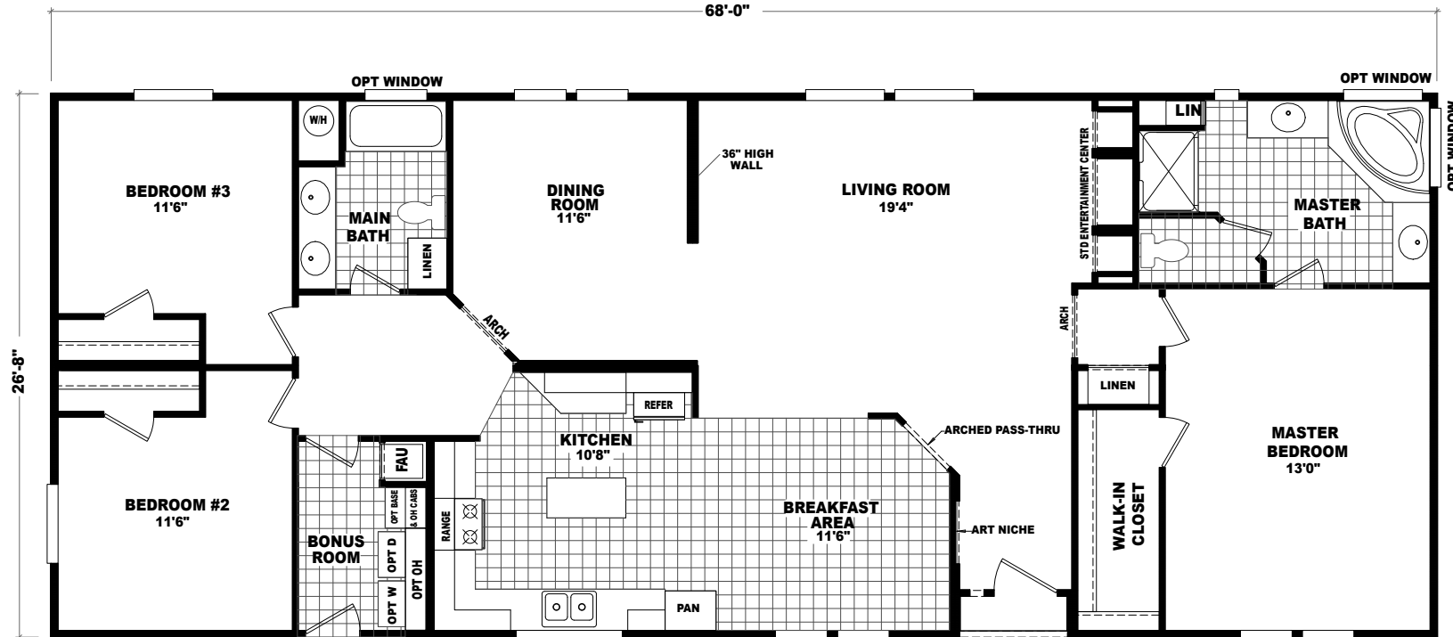
MODEL: DEV-1813A APPROXIMATELY 1813 SQ. FT. 3 BEDROOM, 2 BATH
