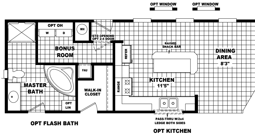
MODEL: CS5628A APPROXIMATELY 1493 SQ. FT. 3 BEDROOM, 2 BATH
