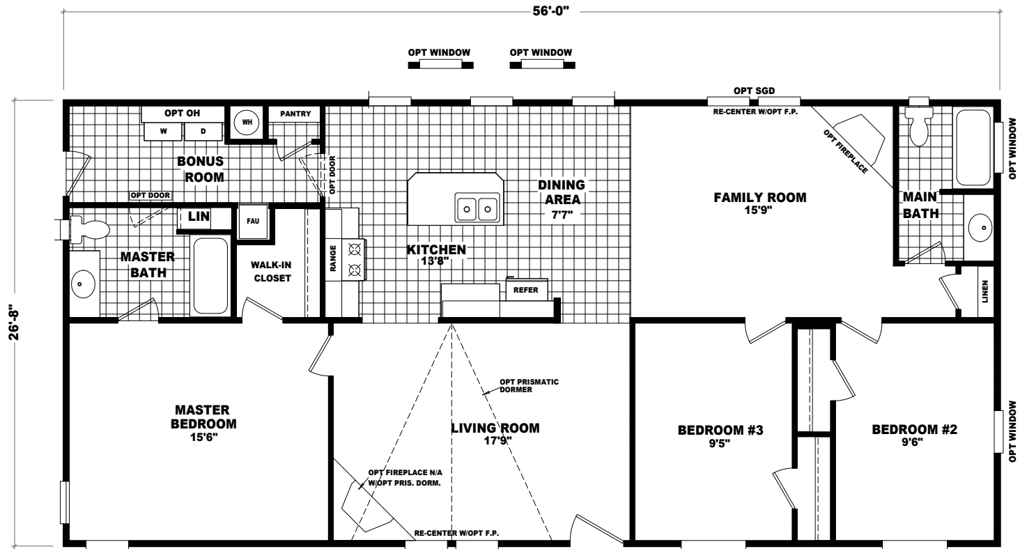
MODEL: CS5628A APPROXIMATELY 1493 SQ. FT. 3 BEDROOM, 2 BATH
